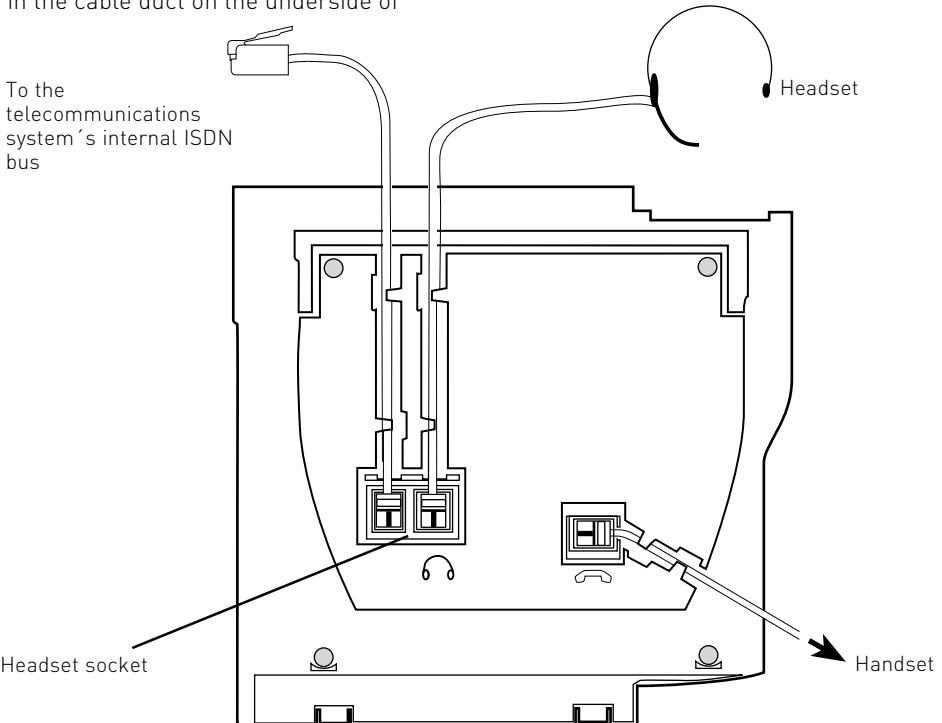
Terminals on the underside of the digital system telephone ST 25
